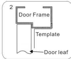
2 Door Frame Template Door leaf Close the door first, then place the upper side of template on door frame, while adjust the left side next to the door leaf. Hollow Metal Door Wooden Door Metal Surface Door
