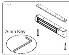
11 Allen Key Use Allen key to screw the lock body on the mounting plate.
