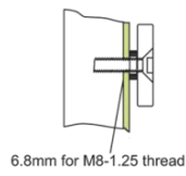
Metal Surface Door Inside: Drill a hole diameter is 8mm folding the plastic straight pin
