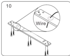
10 Wire Fix the mounting plate on the door frame according to the holes drilled earlier.
